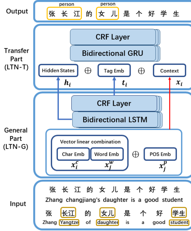
Fig. 1. The light transfer NER model(LTN)
